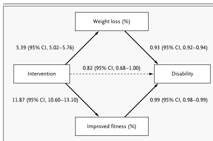
Figure 3. Path Diagram for Mediation Model.
